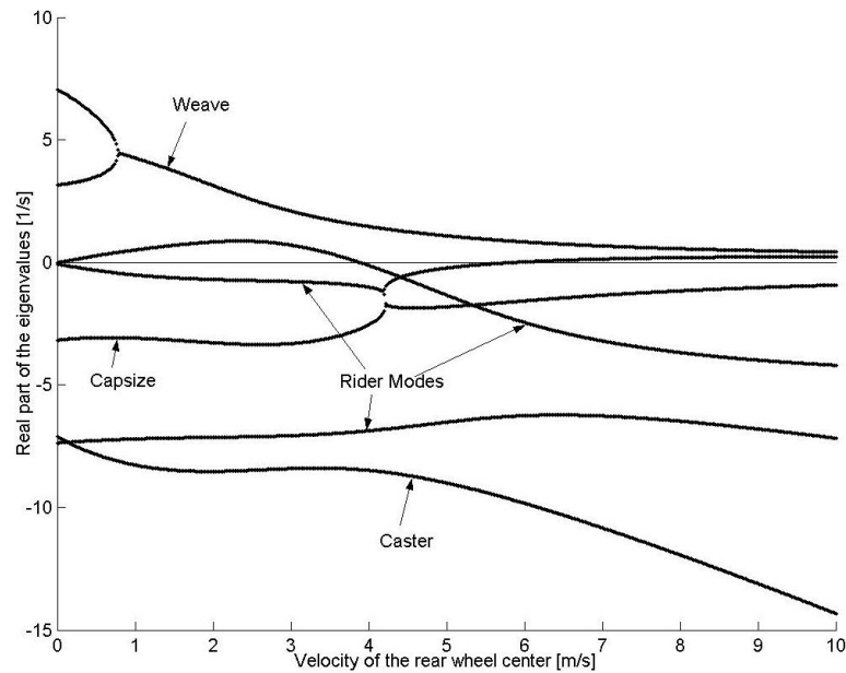
Figure 4.18: Real parts of the eigenvalues as a function of forward speed with the stiffness and damping terms set to realistic values.
