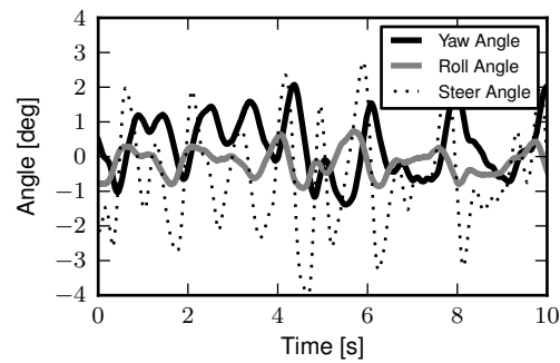
Figure 8.15: The bicycle yaw, roll and steer angles throughout a single a normal biking run at 10 km/h.
