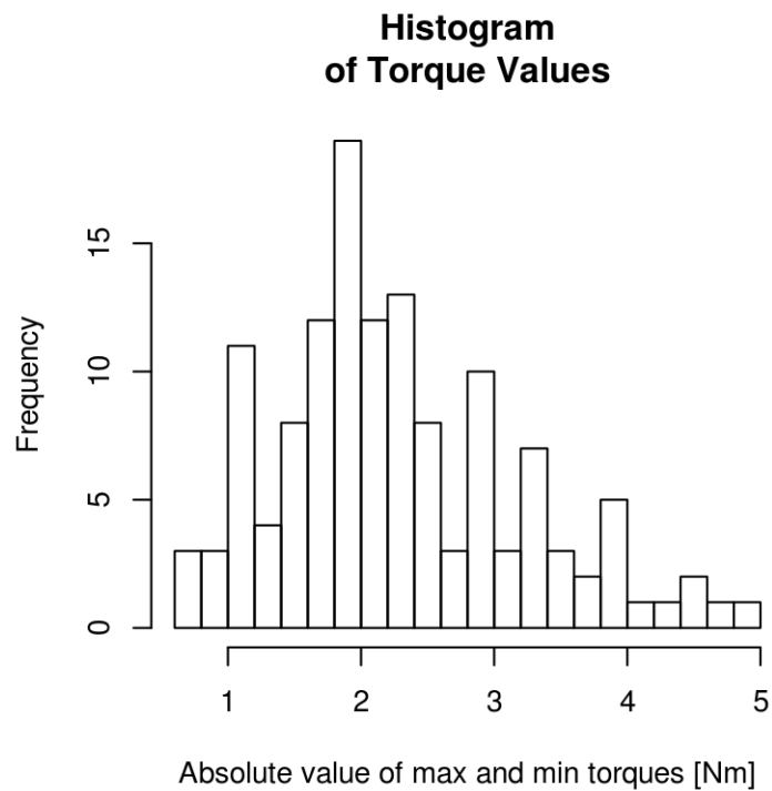
Figure 9.19: A histogram of the maximum recorded torques for all runs. The median is around 2 Nm with torques measured up to 5 Nm. Generated by src/davisbicycle/torque-wrench.R .
