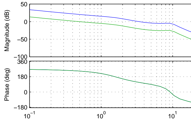
Figure 10.17: The open loop frequency response for the front wheel lateral deviation loop. Blue is gain of unity and the green line uses the gain to give desired crossover. Generated by src/control/choose_gains.m .
