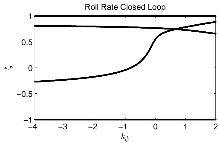
Figure 10.12: The damping ratio of all roots of the roll rate closed loop as a function of gain k_\phi . Generated by src/control/choose_gains.m .
