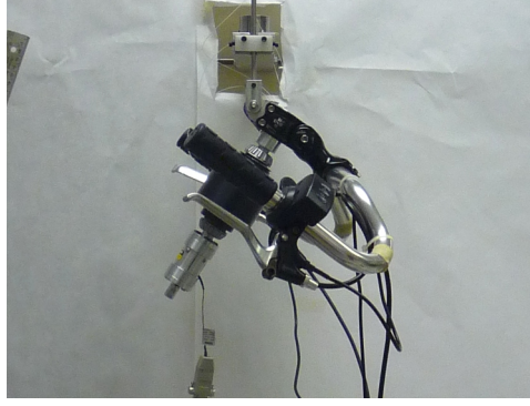
Figure 5.12: The handlebar mounted as a torsional pendulum.
