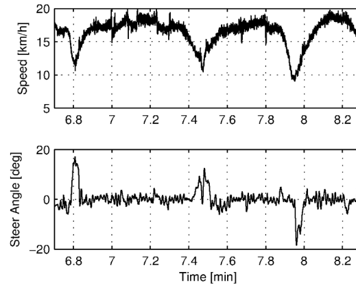
Figure 7.2: Data collected during a ride around town. The upper graph shows the speed the bicycle was traveling at; the lower the steering angle.
