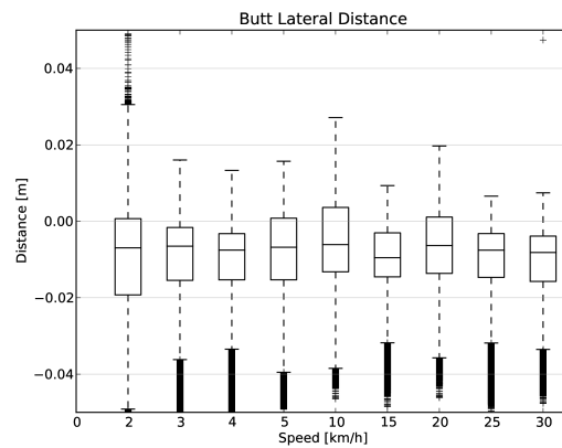
Figure 8.24: Box and whiskers plots of the butt lateral distance data from all riders and bicycles versus speed.
