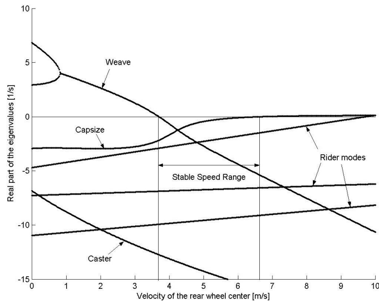
Figure 4.21: Real parts of the eigenvalues as a function of forward speed with the stiffness and damping terms set to unrealistically high values.
