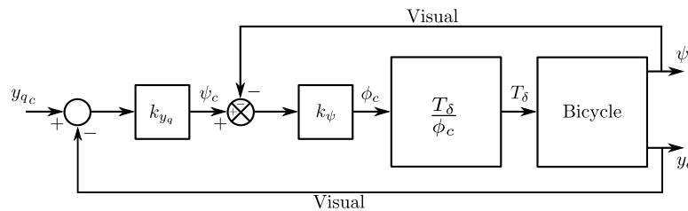
Figure 11.21: The outer loop structure of the control system with the inner loops closed which feeds back the heading \psi and the front wheel lateral deviation y_q .
