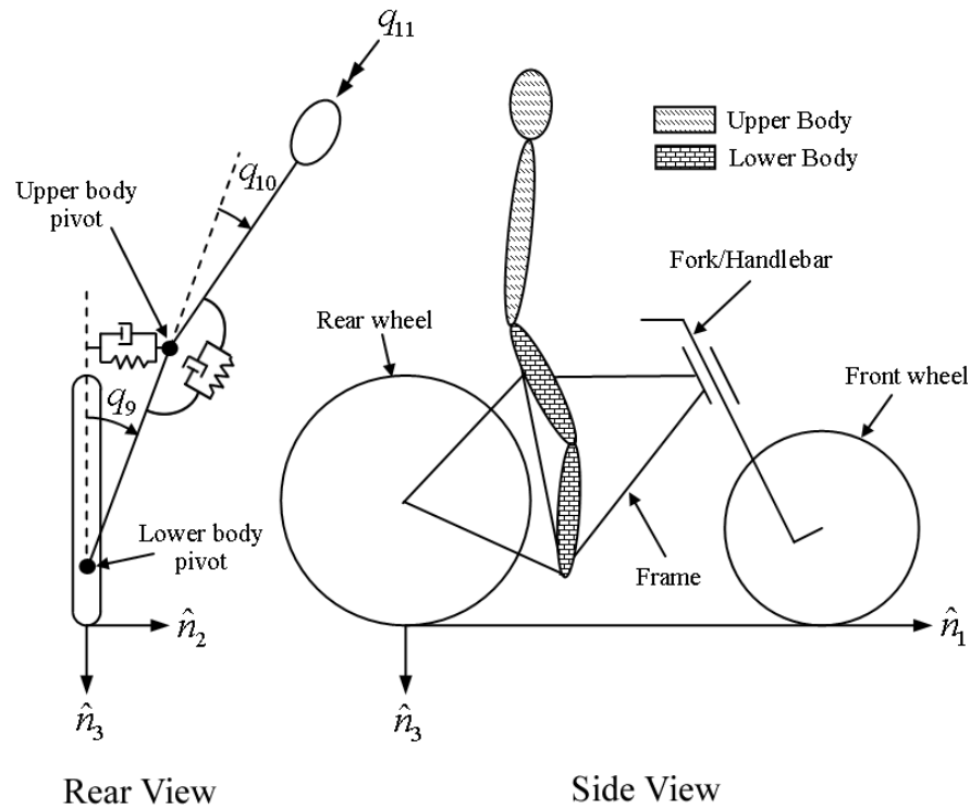
Figure 4.17: Pictorial description of (a) the additional rider degrees of freedom and (b) the six rigid bodies.
