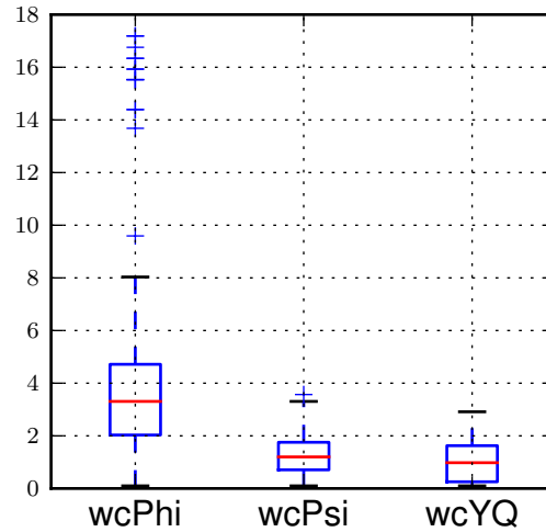
Figure 11.30: Median crossover frequencies in rad/s for the open outer loops for all runs at all speeds.
