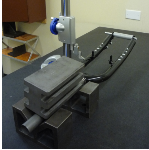
Figure 5.4: The fork of the Davis Bicycle setup for measuring the fork offset.
