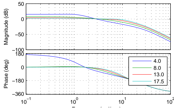
Figure 10.8: The Bode plots of the closed steer loop with various gains. Notice how the higher gains start to increase the bandwidth by pushing the neuromuscular pole closer to a frequency typical of human operator and plant dynamics [HMH12]. Generated by src/control/choose_gains.m .
