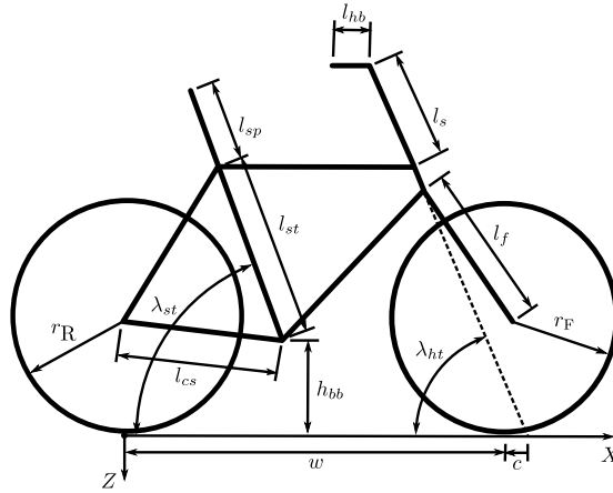
Figure 5.23: The dimensions need to construct the grid point system in the simple inertia method.
